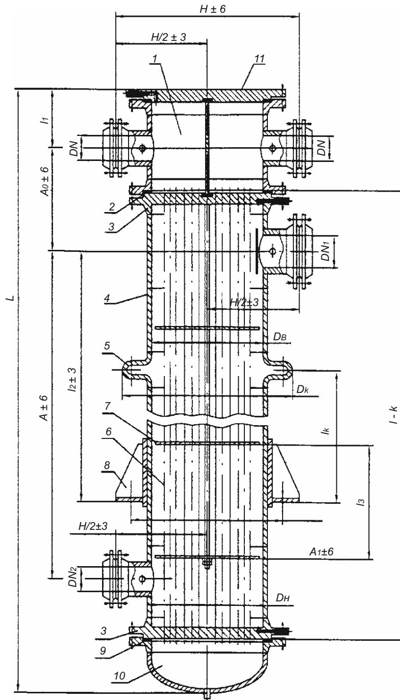
Multi-pass through tubes heat exchangers of KNV, KKV types
