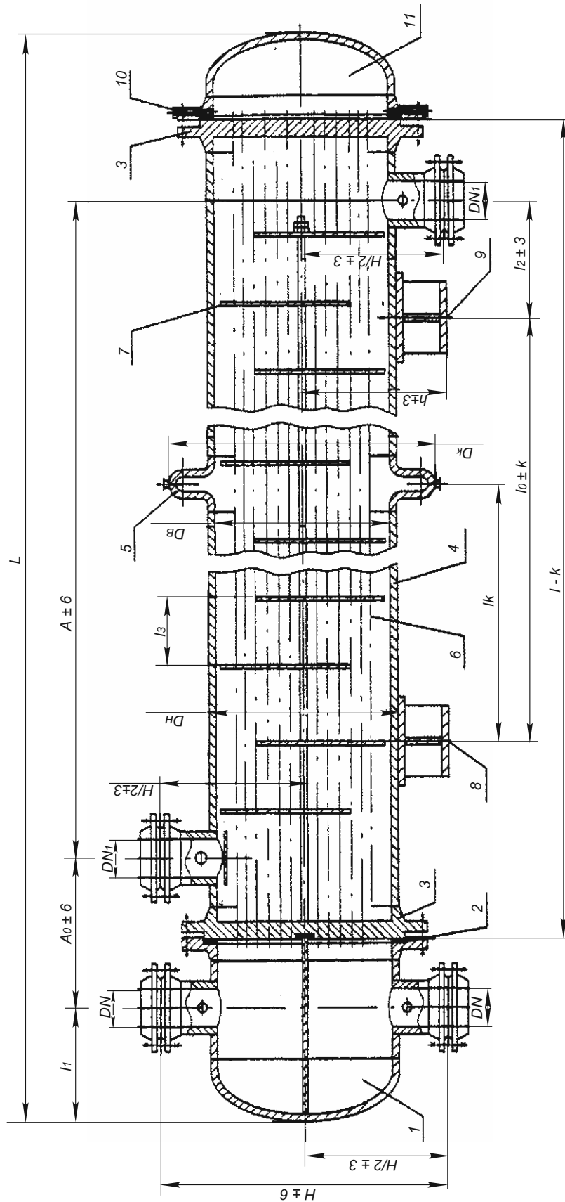
Multi-pass through tubes heat exchangers of TNG, TKG types
