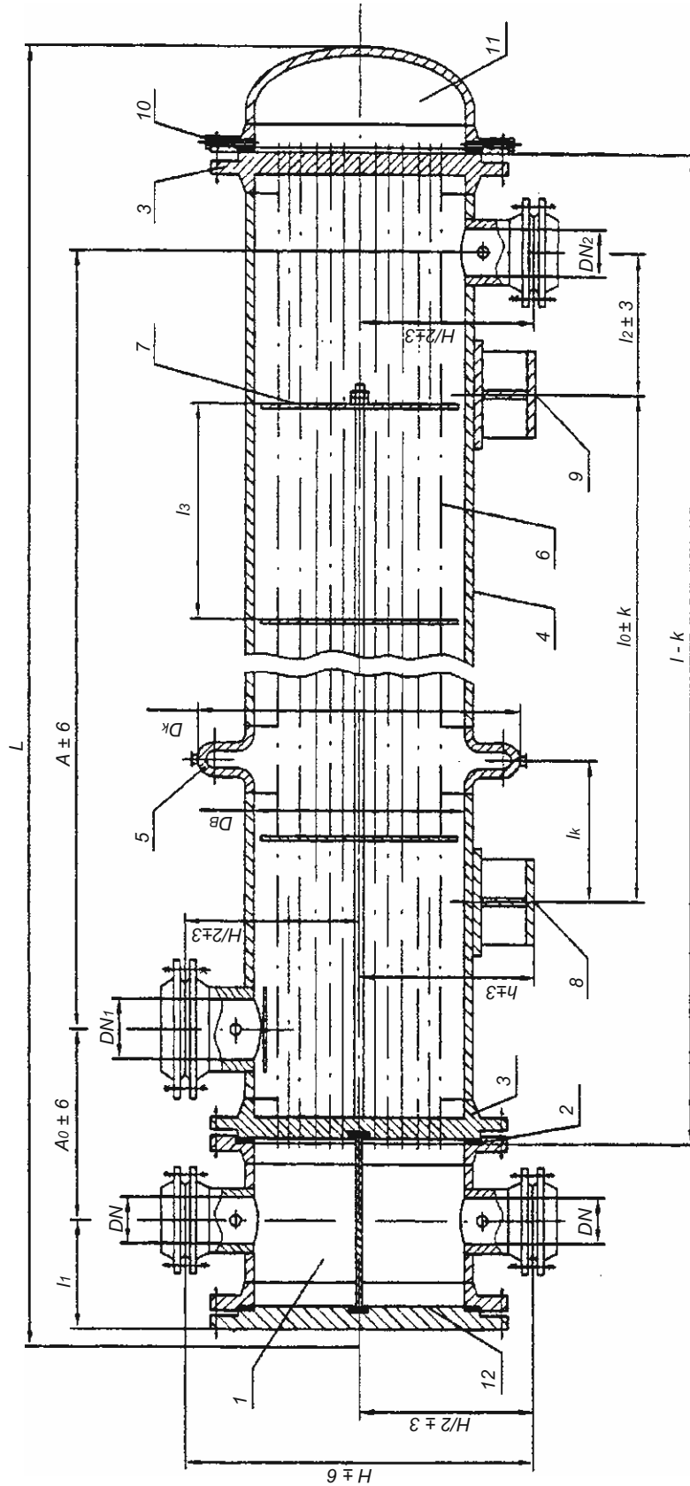
Multi-pass through tubes heat exchangers of KNG, KKG types
