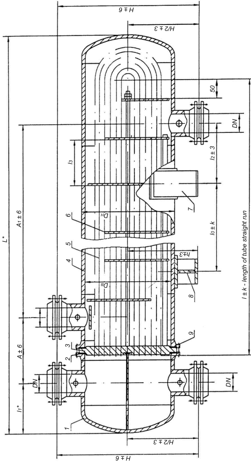
Heat exchanger of TU type
