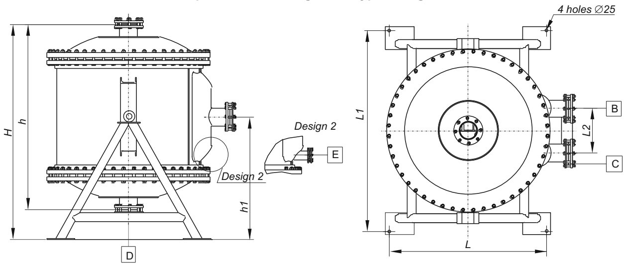
Spiral heat exchanger of 2 type, design 1
